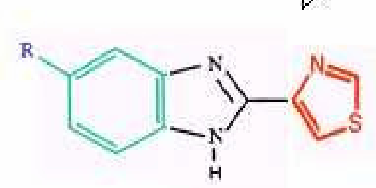
Benzimidazoles
