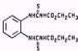
Thiophanate
